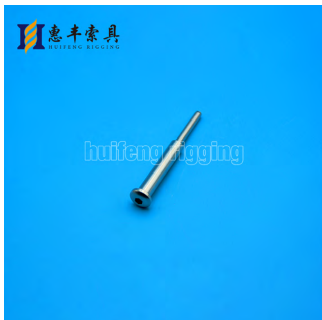
圆头隐形内六角套件 Dome Head Invisible Receiver and Swage Stud
